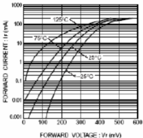
Fig.1 Forward characteristics
