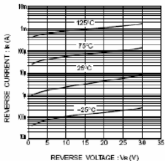
Fig.2 Reverse characteristics
